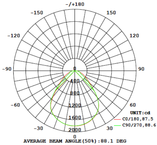
Very Wide (90°) at 36W 3000K
