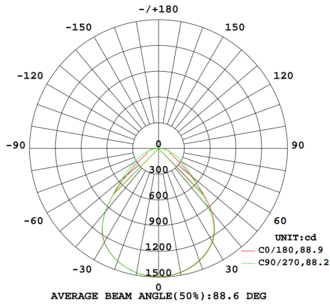
Wide (90°) at 20W 3000K
