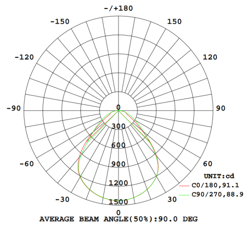
Wide (90°) at 20W 4000K
