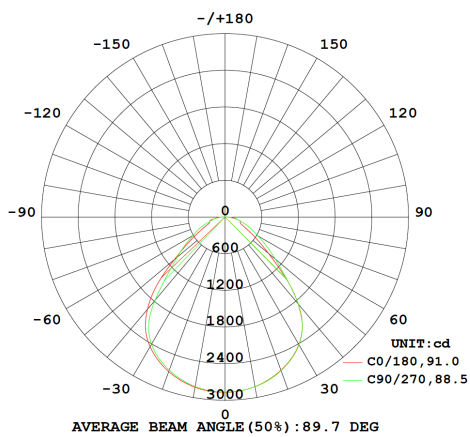
Wide (90°) at 60W 3000K
