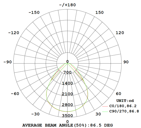
Wide (90°) at 60W 4000K
