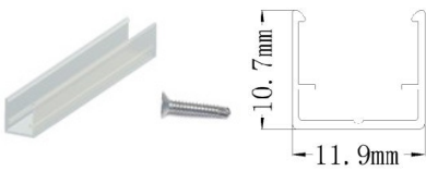
LPA-NF-TC10-Mounting Aluminium mounting profile & screw
