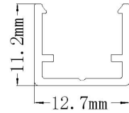
LPA-NF-TC10-Clips Mounting clips
