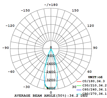
Medium (34°) at 21W
