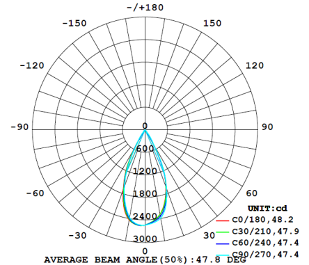
Wide (48°) at 21W
