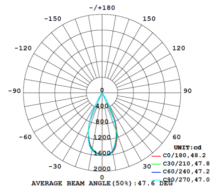
Wide (48°) at 13W
