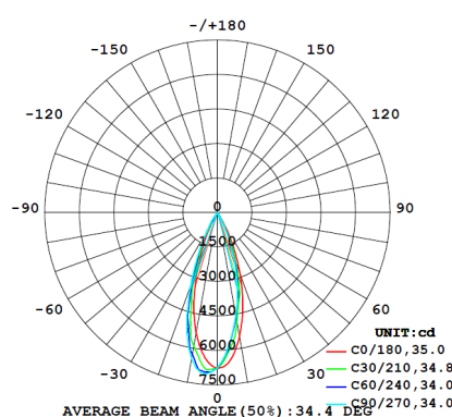
Medium (34°) at 31W
