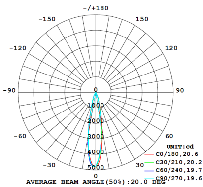
Narrow (20°) at 13W
