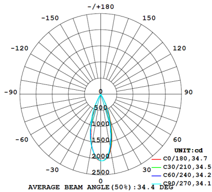
Medium (34°) at 13W
