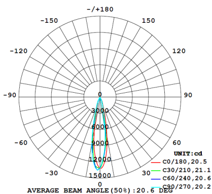
Narrow (20°) at 31W
