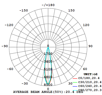
Narrow (20°) at 21W
