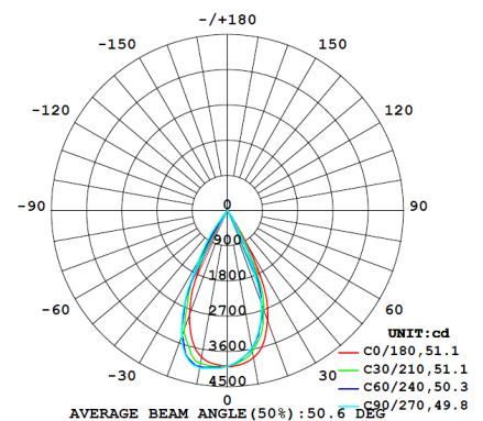
Wide (48°) at 31W
