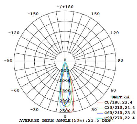
Narrow (24°) at 8W
