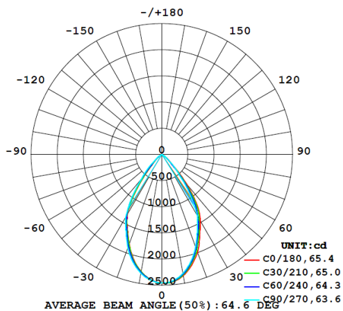
Wide (65°) at 27W
