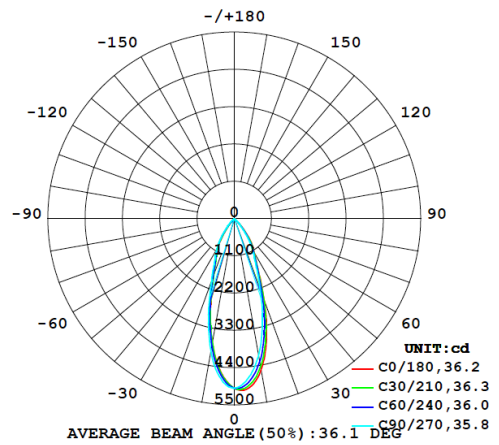
Medium (36°) at 27W
