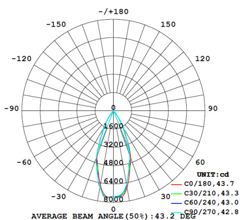
Medium (43°) at 39W
