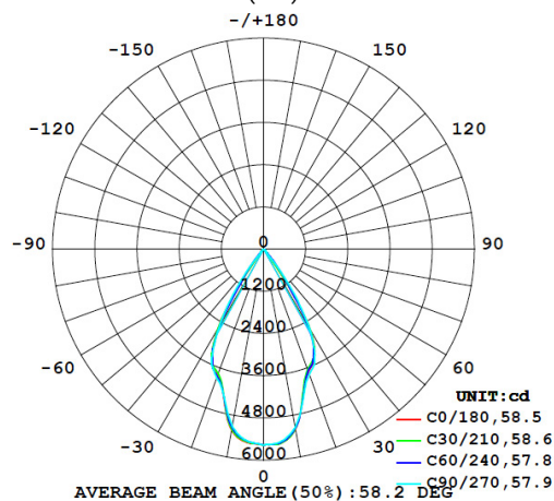
Wide (58°) at 39W
