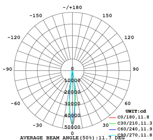
Narrow (12°) at 39W
