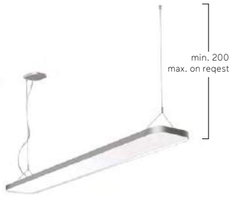
Y-Cord Suspension
