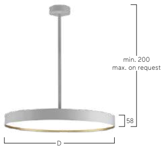
Tube Suspension
