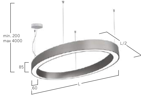
Parallel Suspension
