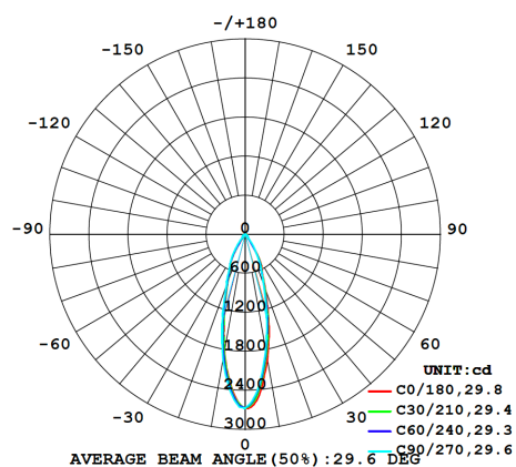
Medium (30°) at 15W
