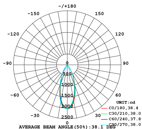
Medium (38°) at 15W
