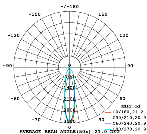
Narrow (21°) at 15W
